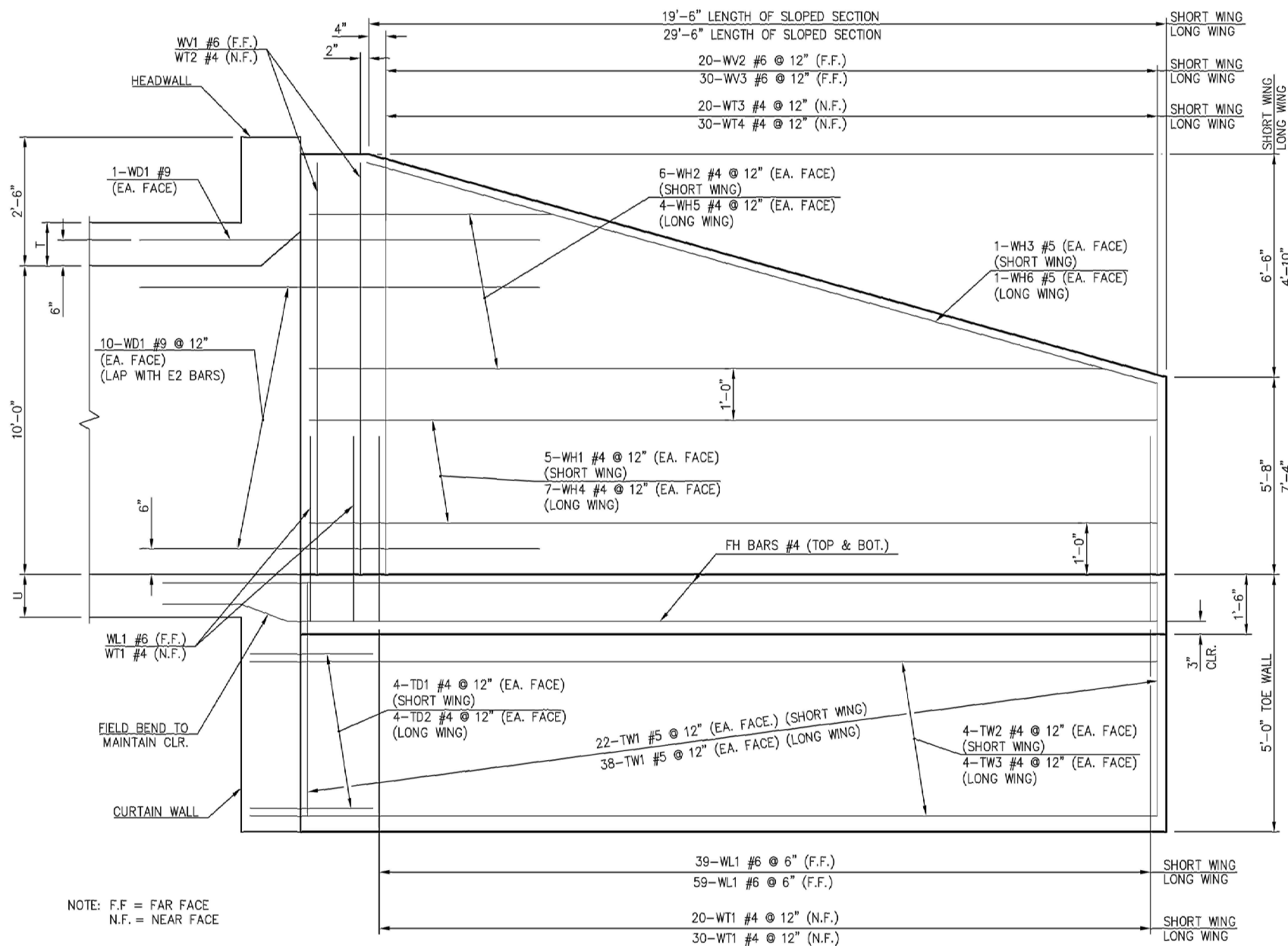
WING ELEVATION
